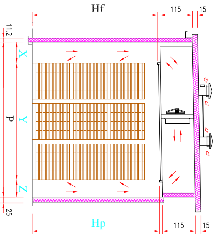
SIDE VIEW IN SECTION
